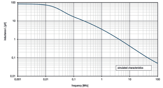
Fig. 4: Inductance L i [μH] / frequency [MHz]
