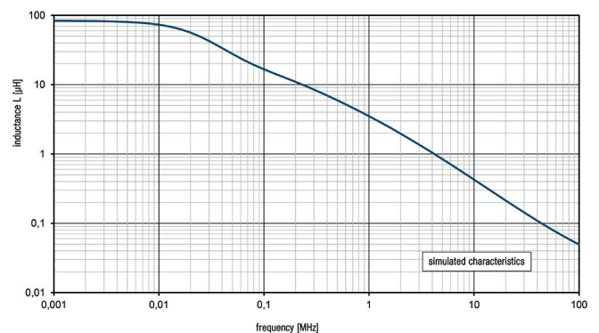
Fig. 2: Inductance L [μH] / frequency [MHz]
