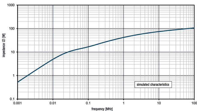
Fig. 1: Impedance |Z| [Ωm] / frequency [MHz]
