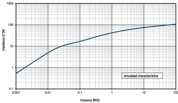
Fig. 3: Impedance |Z| [Ω] / frequency [MHz]
